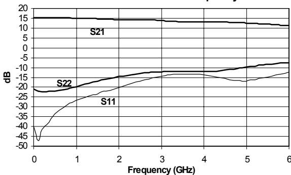
Gain and Return Loss vs Frequency
